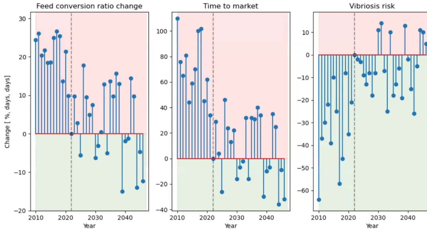
Dicentrarchus labrax - Simulation results for location (43.99, 14.78) - RCP4.5
